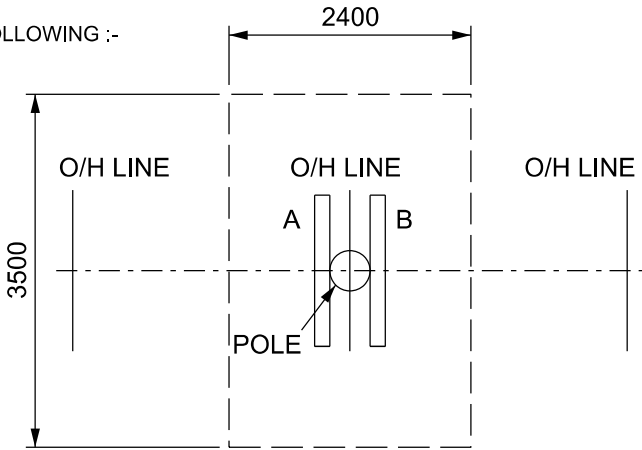
PLAN VIEW TYPICAL FOUNDATION DETAILS FOR SINGLE POLE INTERMEDIATE STRUCTURE
